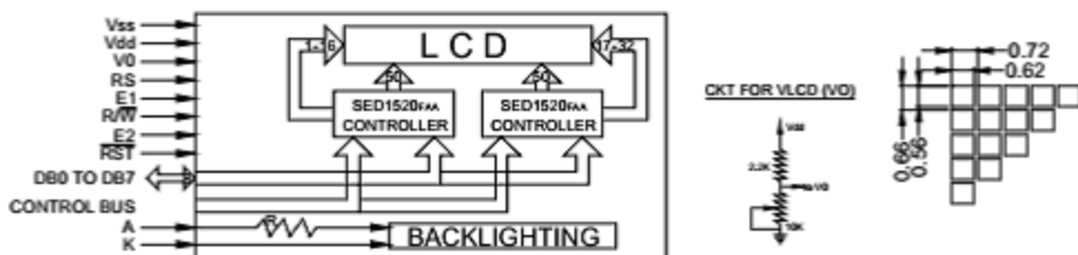
BLOCK DIAGRAM
